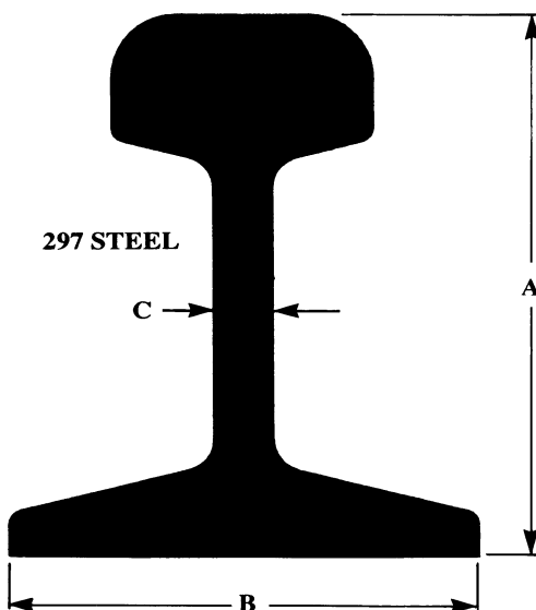
298 STEEL
